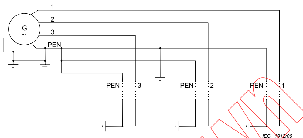
Figure 4 – Three phase system output, single phase distribution
