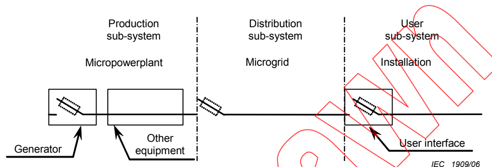
Figure 1 – Microgrid limits
