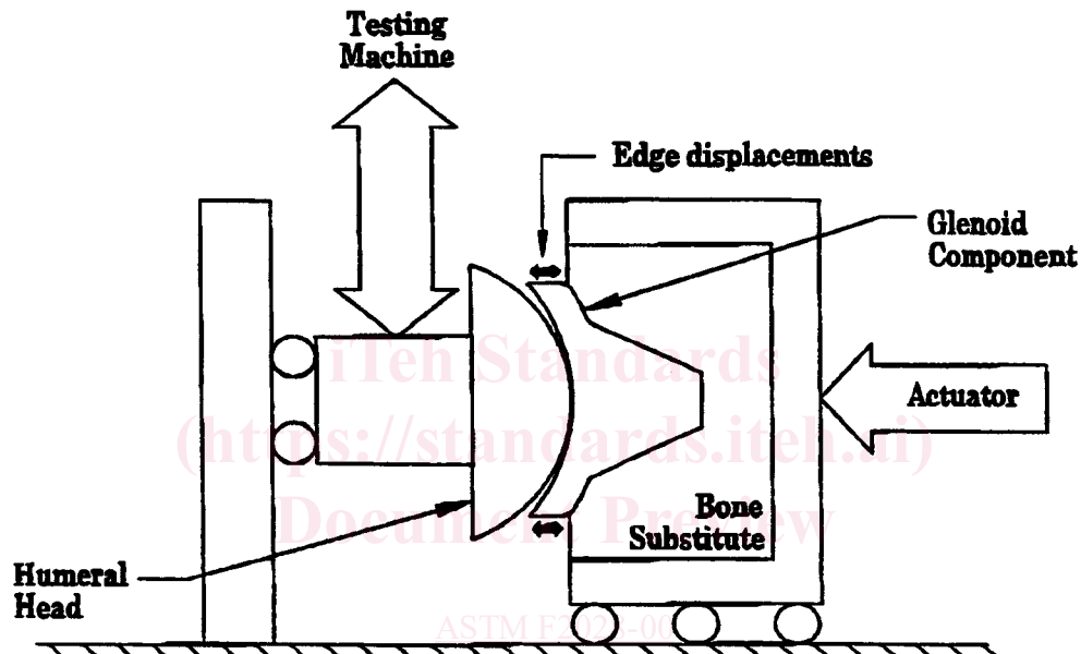
FIG. 3 Biaxial Testing Apparatus
