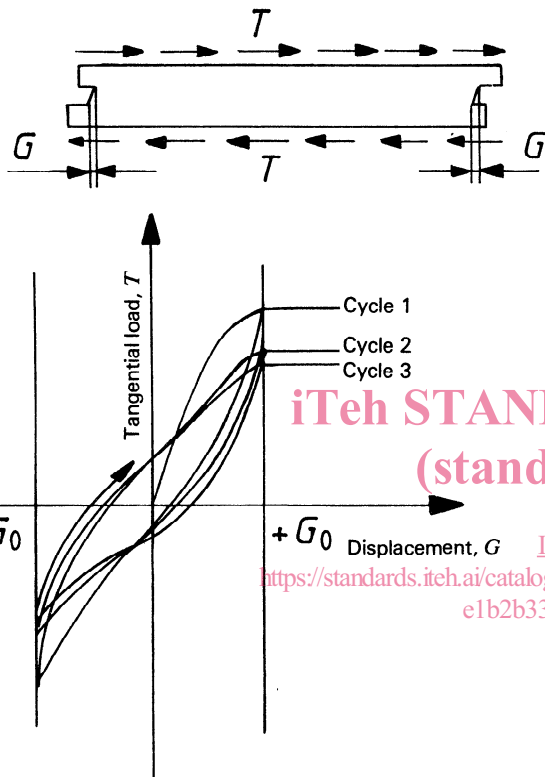
Figure 4 — Example of tangential load-displacement diagram for an alternating shear test with imposed displacement
