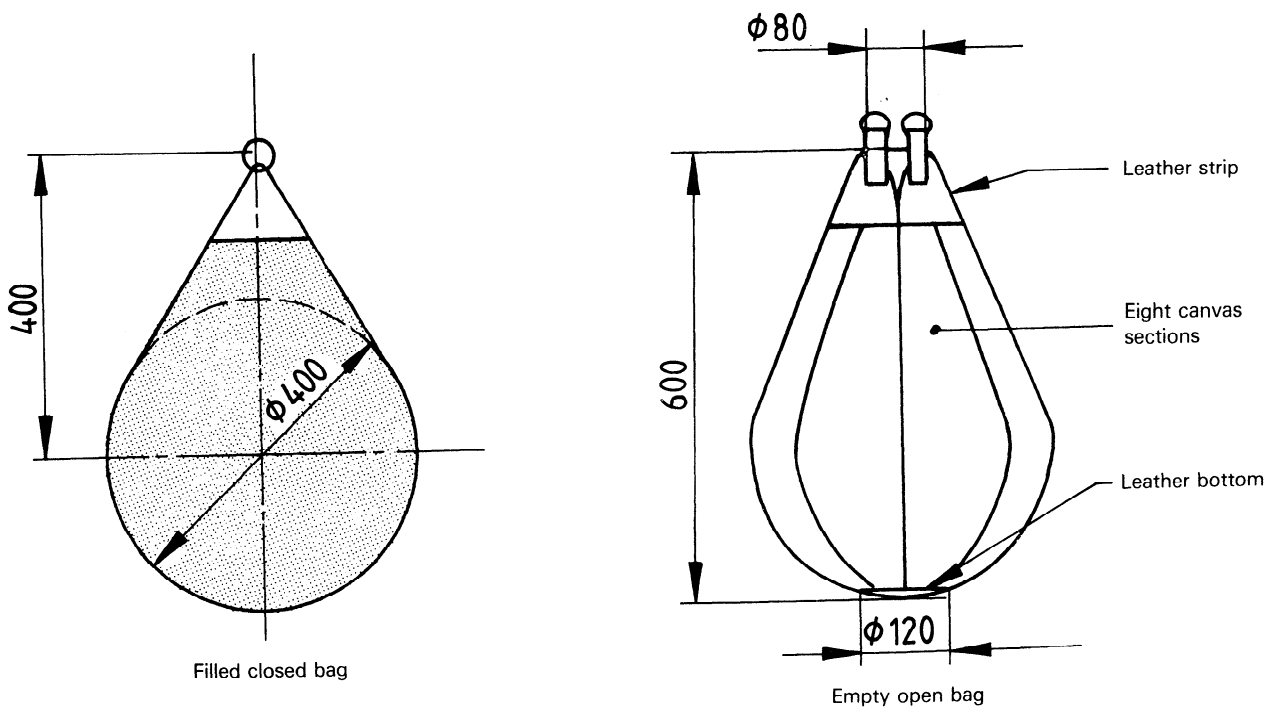
Figure 2 — 50 kg spheroconical bag
