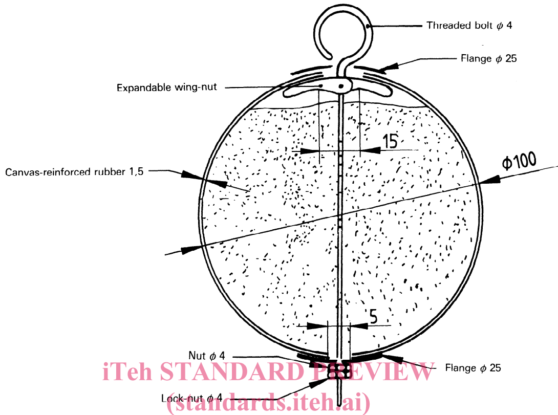
ISO 7892:1988 https://standards.iteh.ai/catalog/standards/sist/c601417-d464-4ba5-b828-4410535aadee/iso-7892-1988 Figure 1 — 3 kg ball
