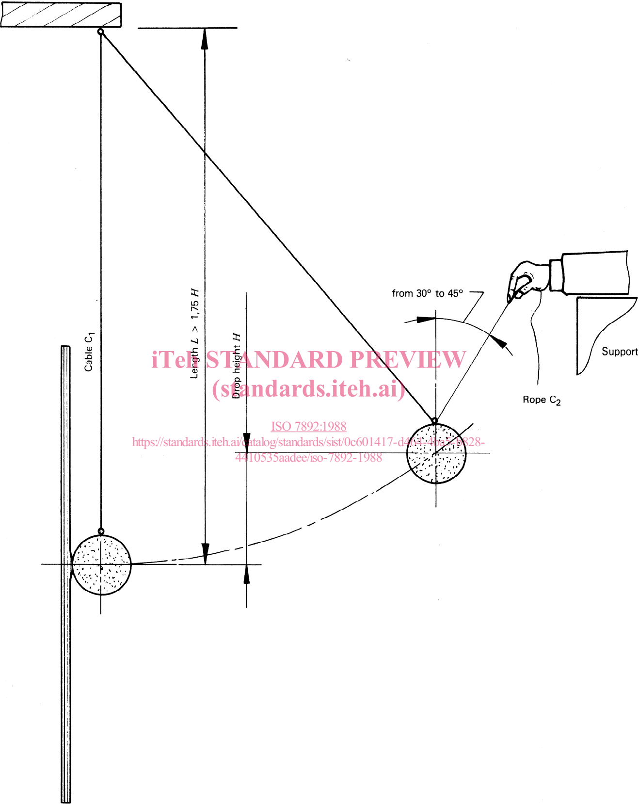
Figure 3 — Example of test apparatus using a small hard impact body
