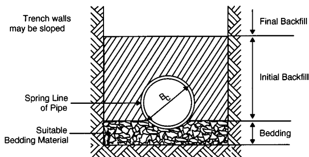
TRENCH CROSS SECTION
