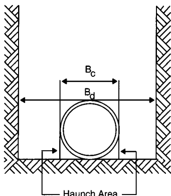
TRENCH CROSS SECTION
