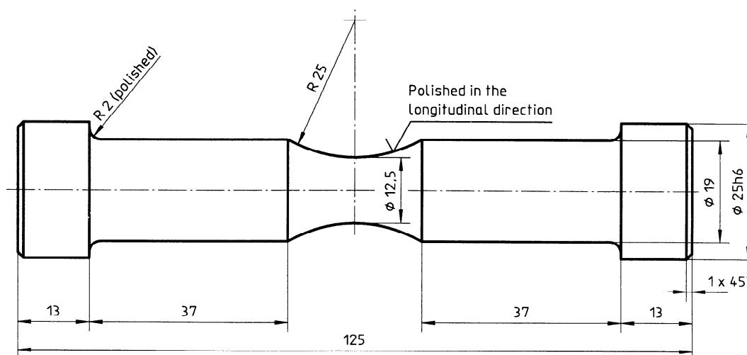
Figure 1 — Specimen dimensions
