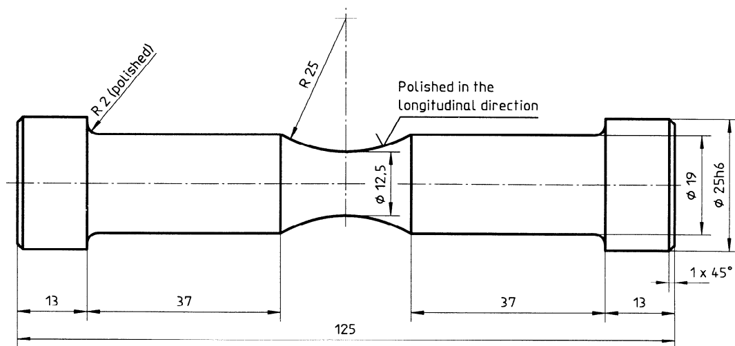
Figure 1 — Specimen dimensions
