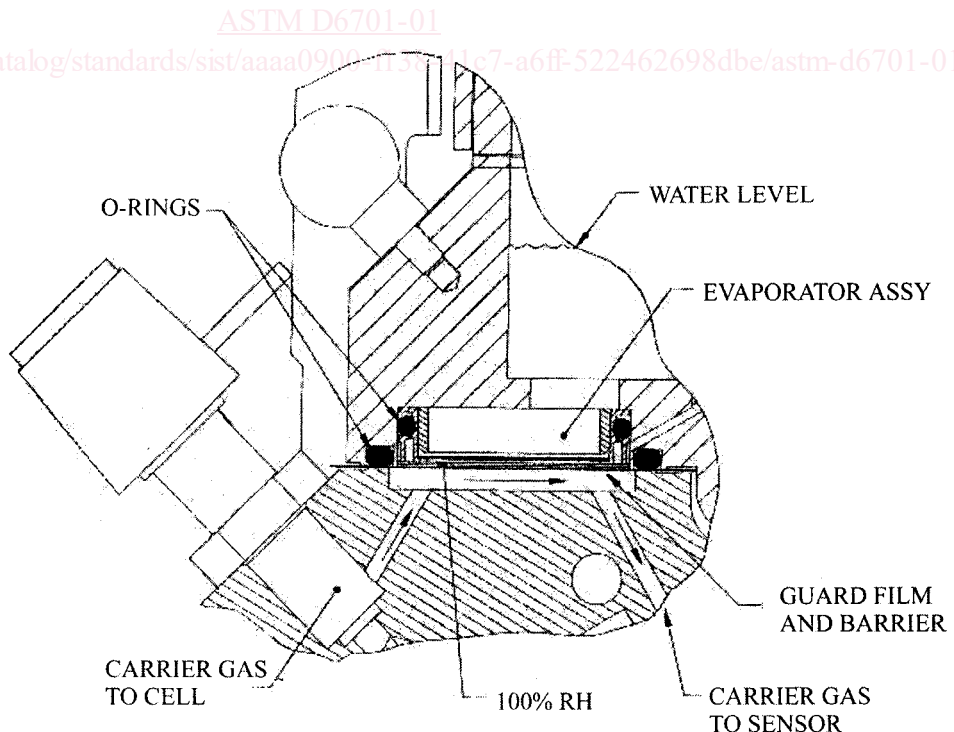
FIG. 1 Typical Cell Cross Section
