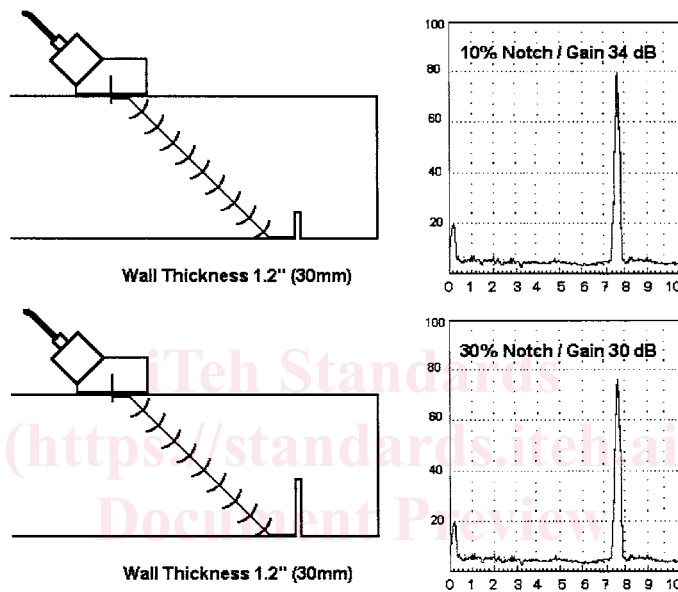
FIG. 5 Generation of Far-Surface Creeping Wave Signal
