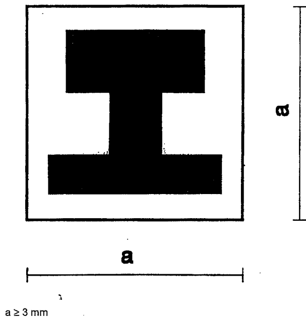
Figure 12(l) — Design mark for isolated gripping-lugs iteh STANDARD PREVIEW (standards.iteh.ai)
