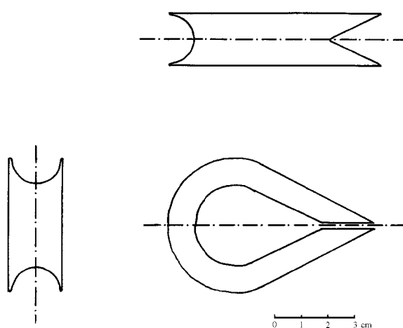
Figure 2 – Example of attaching device
