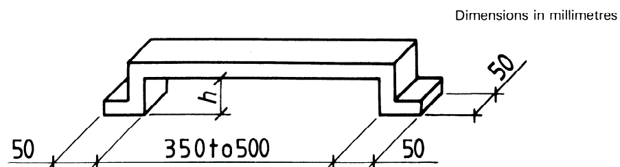
Figure 2 — Steel shackle
