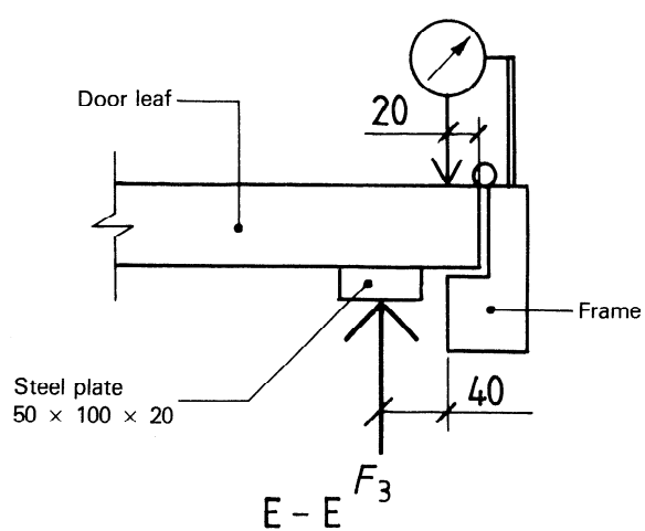
Figure 5 — Testing the hinge side of the door leaf
