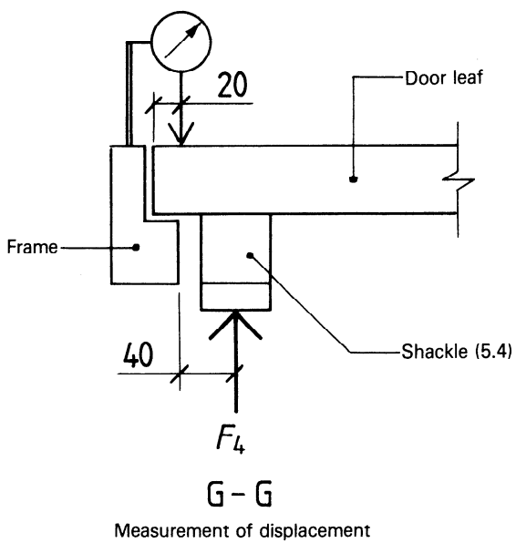
Figure 6 — Testing on lock side
