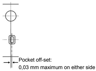
Figure 1 – Type VI carrier tape
