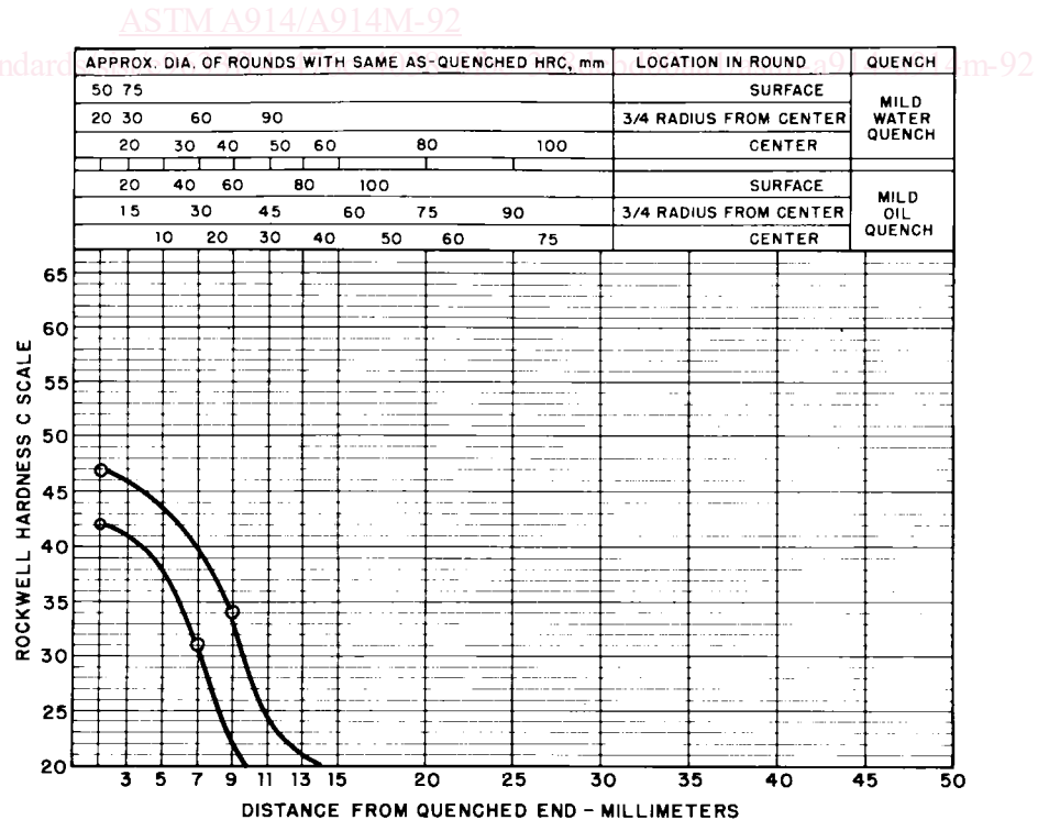
FIG. 2 Limits for Hardenability Band 15B21 RH
