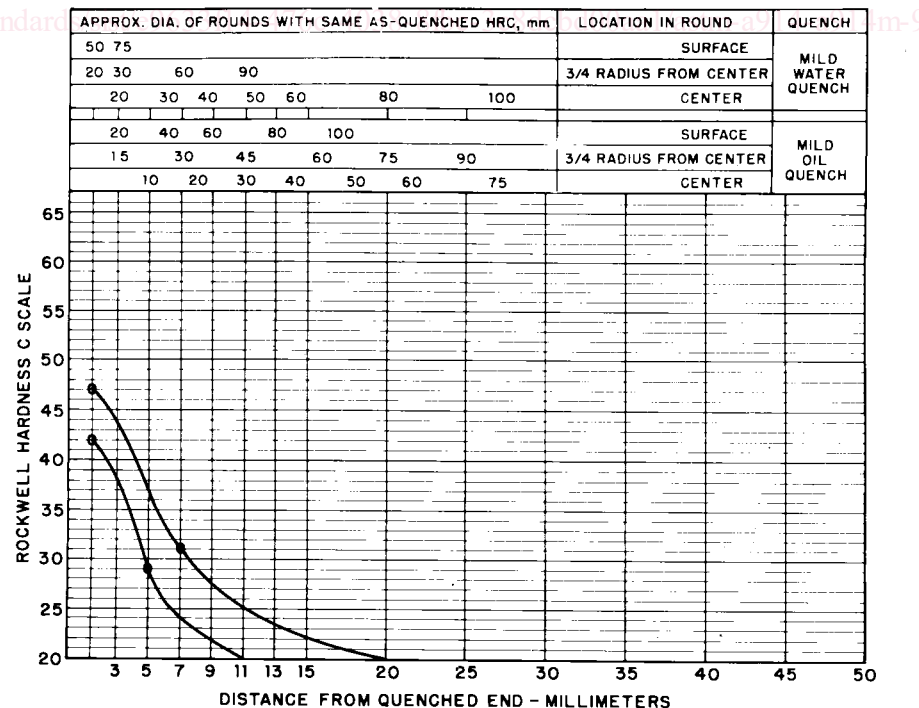
FIG. 6 Limits for Hardenability Band 4118 RH
