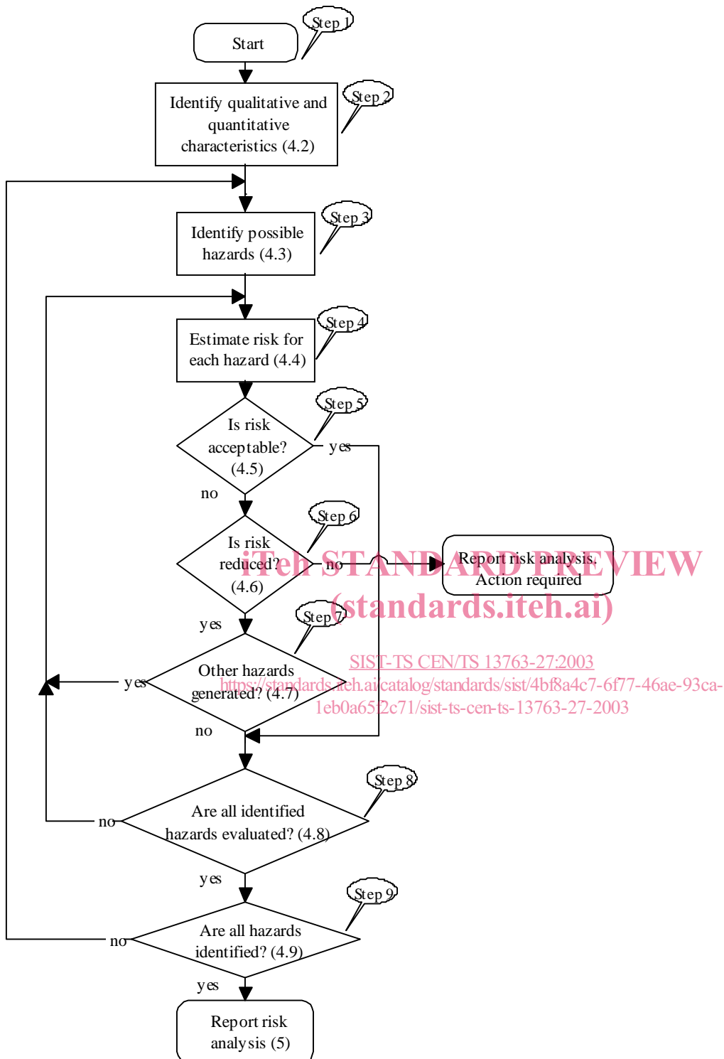
Figure 4 - Flow diagram of risk analysis, evaluation and testing procedure
