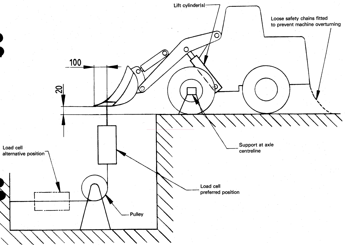
Figure 2 — Typical test arrangement for determination of maximum breakout force exerted by lift cylinder(s)
