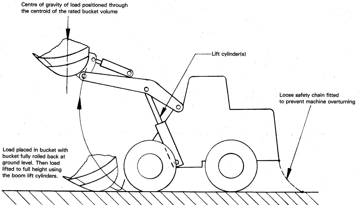
Figure 4 — Typical test arrangement for determination of maximum lifting capacity to full height
