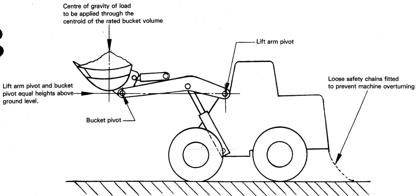
Figure 5 — Typical test arrangement for determination of maximum tipping load at maximum outreach
