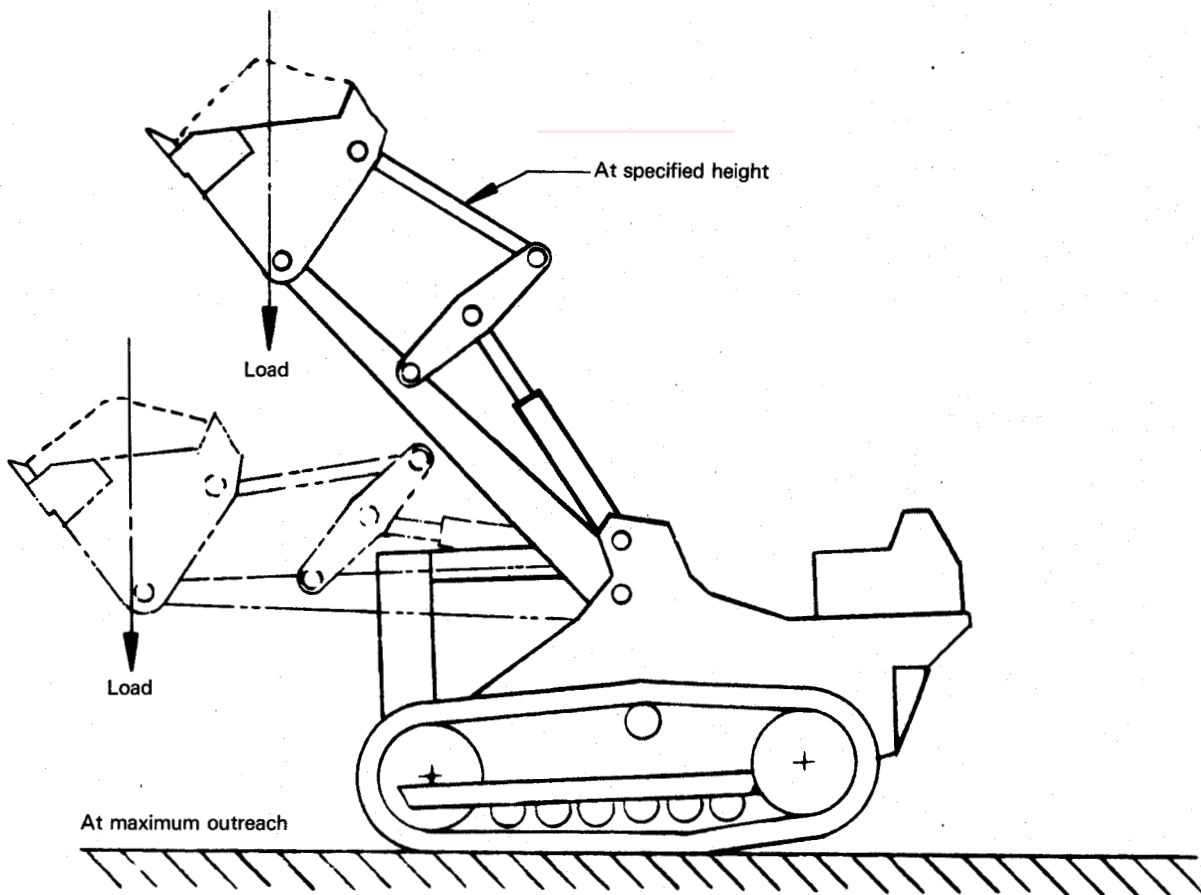
Figure 1 – Tipping condition
