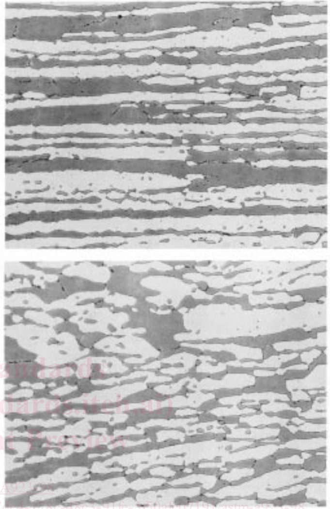
FIG. 2 Possibly Affected Structure in S31803: (a) Longitudinal Section and (b) Transverse Section (500× Magnification Before Reproduction)
