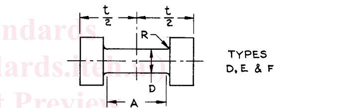
FIG. 2 Alternative Tension Test Specimens
