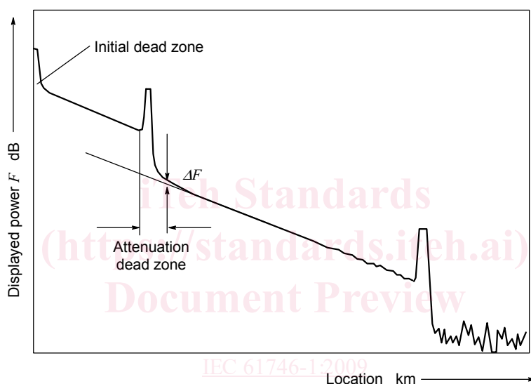
Figure 1 – Definition of attenuation dead zone
