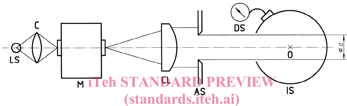
a) Using a collimator lens
