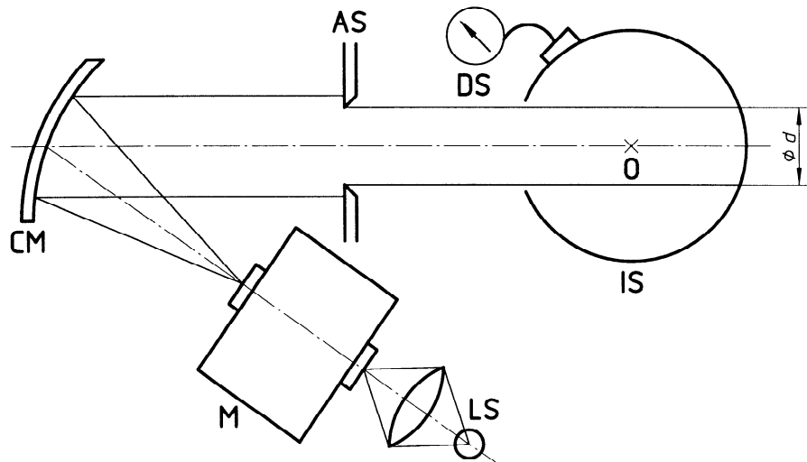
b) Using an off-axis paraboloid mirror collimator
