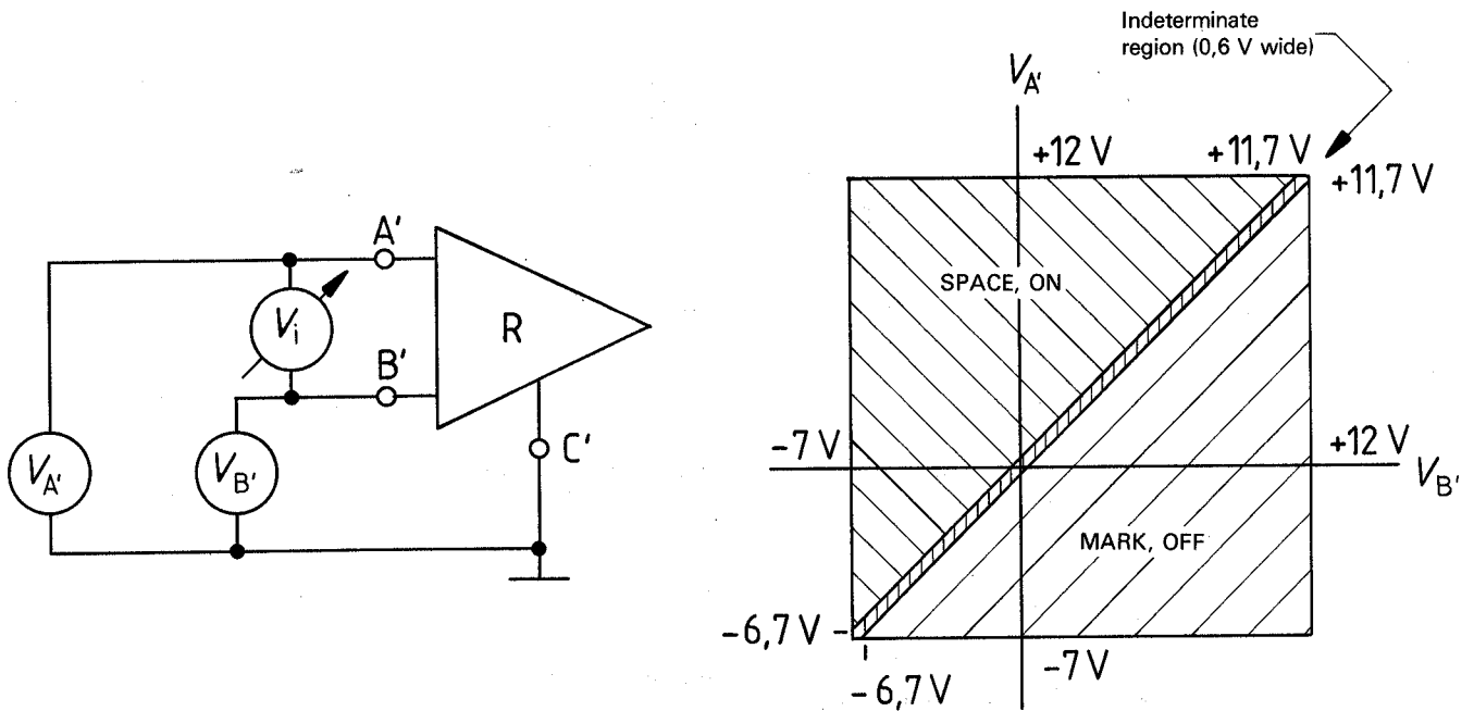
iTeh STANDARD PREVIEW Figure 11 – Input voltage range (standards.iteh.ai)
