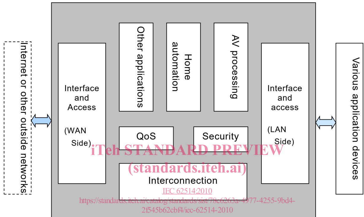
Figure 2 – HMG architecture
