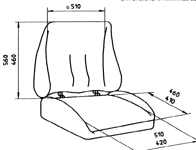
Figure 2 — Seat dimensions
