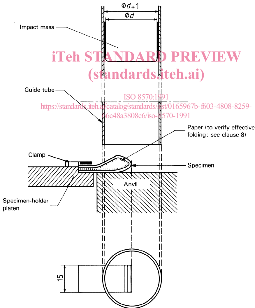
Figure 1 — Typical impact device for determination of cold-crack temperature
