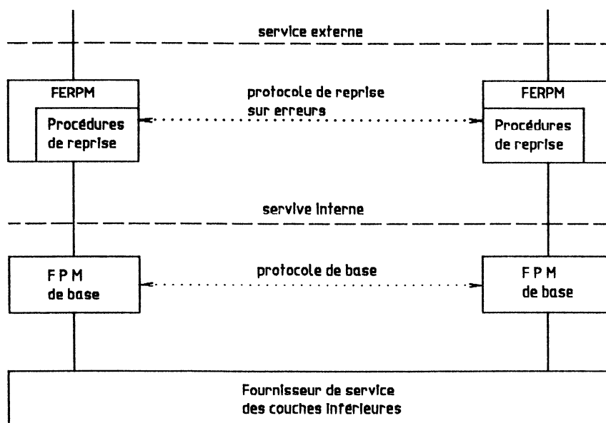
Figure 1 — Niveaux de service
