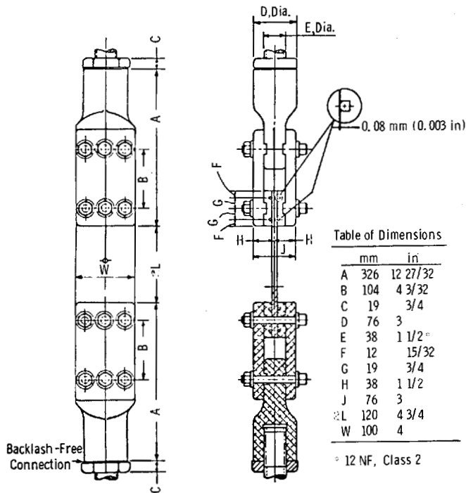
FIG. 4 Example of Bolt and Keyway Assembly for Gripping 100-mm (4-in.) wide M(T) Specimen
