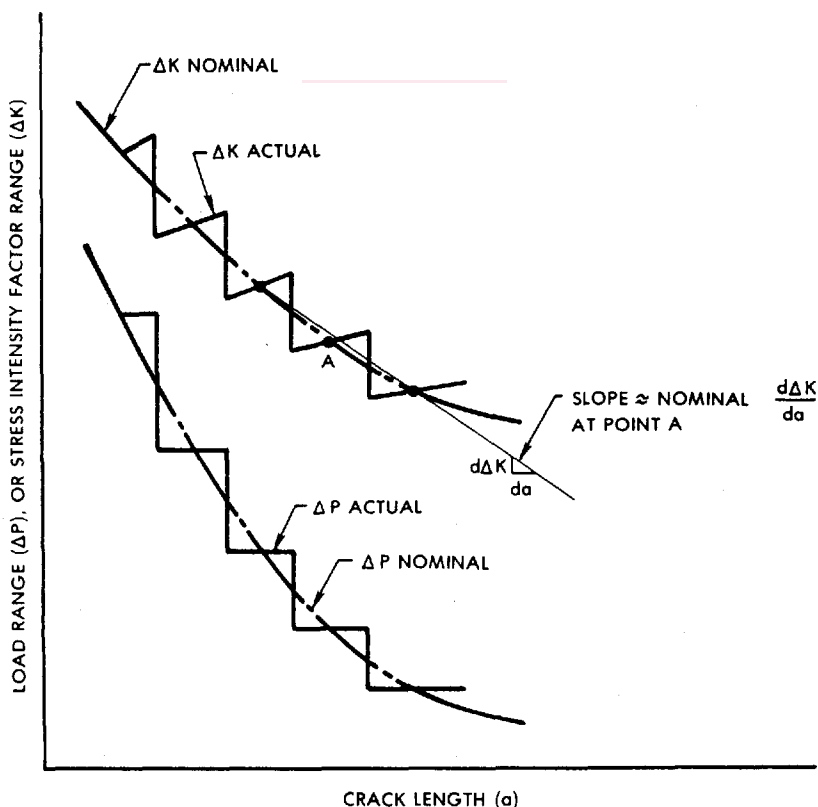
FIG. 7 Typical K Decreasing Test by Stepped Load Shedding
