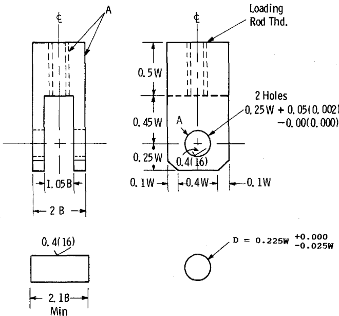
FIG. 3 Clevis and Pin Assembly for Gripping C(T) Specimens
