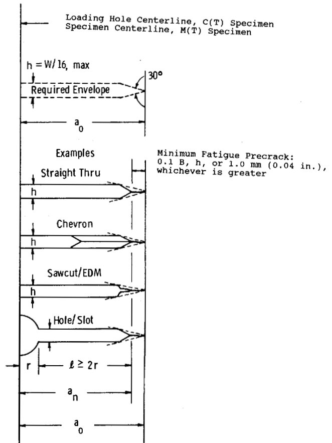
FIG. 5 Notch Details and Minimum Fatigue Precracking Requirements
