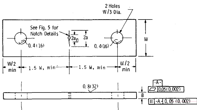
FIG. 1 Standard Compact-Tension C(T) Specimen for Fatigue Crack Growth Rate Testing
