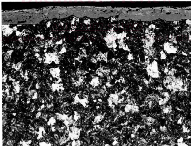
FIG. 4 Example of an As-Rolled, Fully Pearlitic Alloy Steel Microstructure With No Apparent Decarburization. Dark Layer at Surface Is Iron Oxide (Mill Scale) (200×, 2 % Nital Etch)
