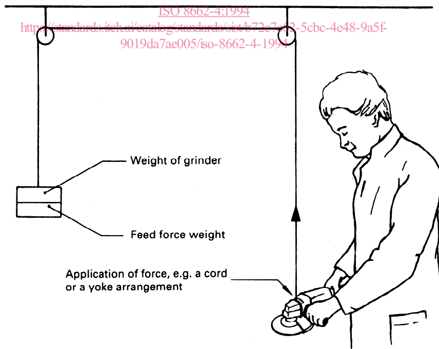
Figure 3 — Grinder — Working position of operator
