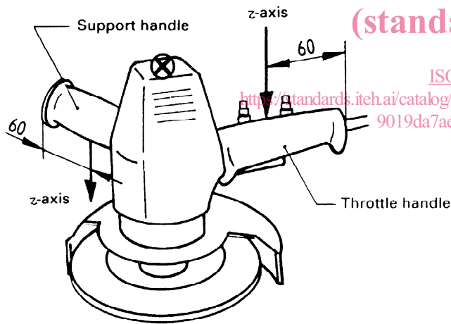
Vertical grinder
