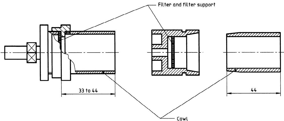
Figure 1 — Filter holders
