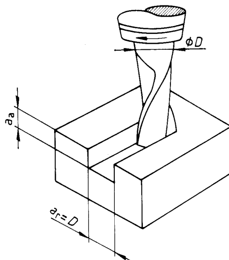
Figure 1 — Rainurage
