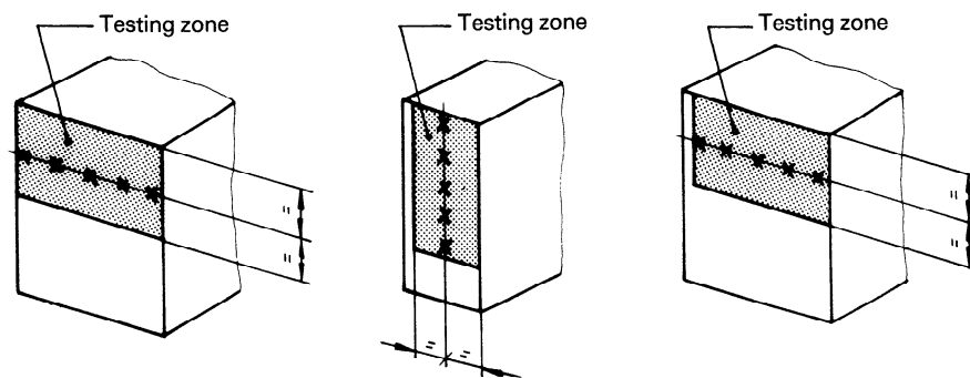
Figure 4 – Hardness testing
