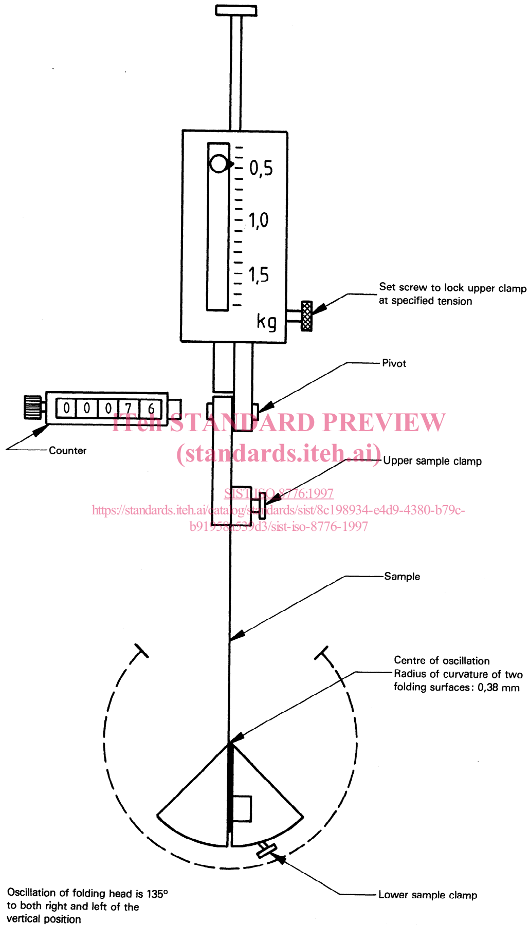
Figure — Operating mechanism of the MIT folding endurance tester
