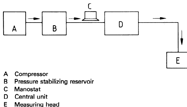
Figure 1 — Circuit diagram of test apparatus
