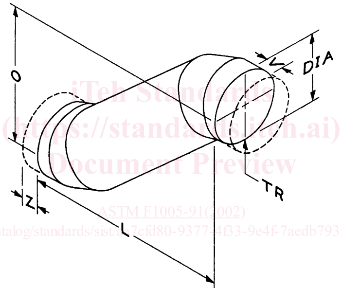
FIG. 4 Shape 2.1—Offset-Round
