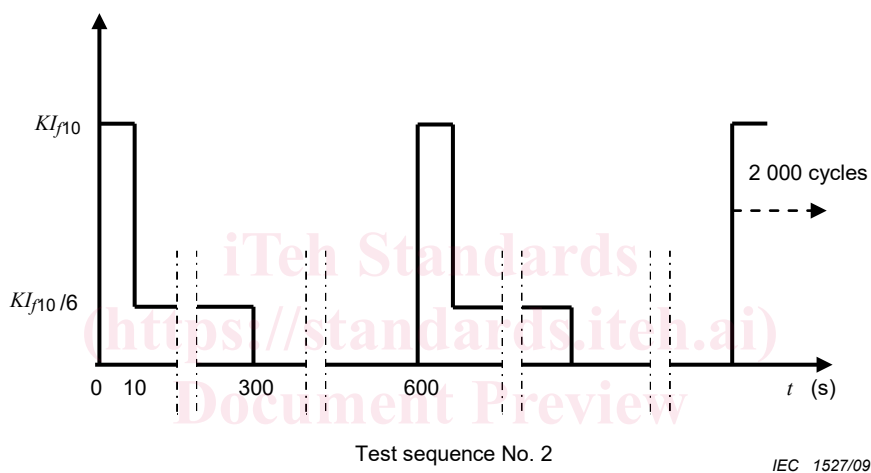
https://standards.iteh.ai/catalog/standards/iec/60644-2009 Figure 1 – Diagrams of the test sequences 5f190d384/iec-60644-2009
