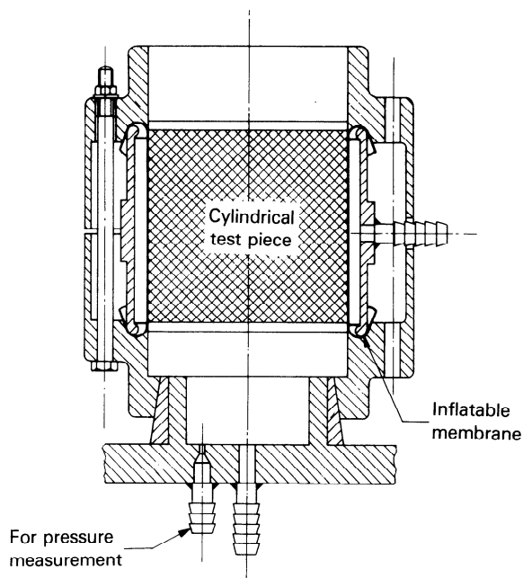
Figure 3 — Test piece holder
