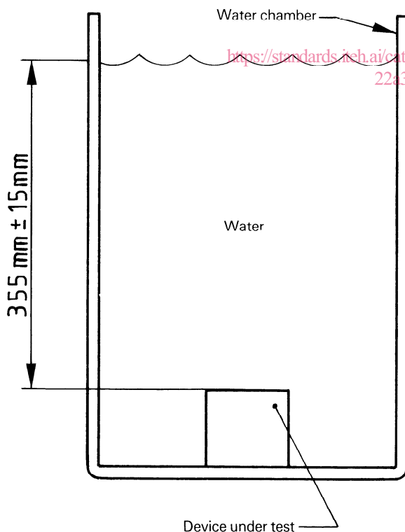
Figure 1 — Water chamber for sealed devices
