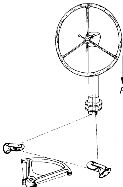
Figure 4 — Application de la charge tangentielle
