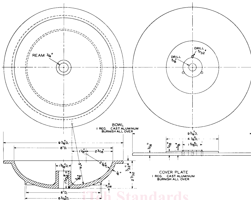
NOTE 1—See Table 2 for metric equivalents. FIG. 1 Extraction Unit Bowl (Test Method A)
