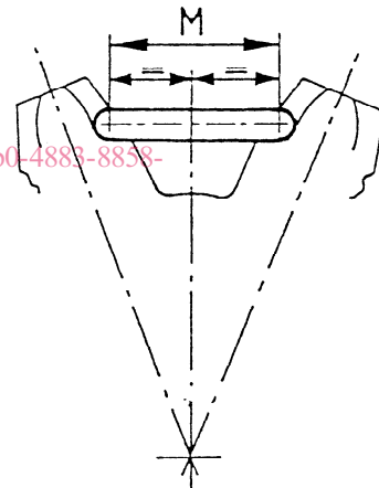
FIGURE 8 - Pocket centres (Dimension M)
