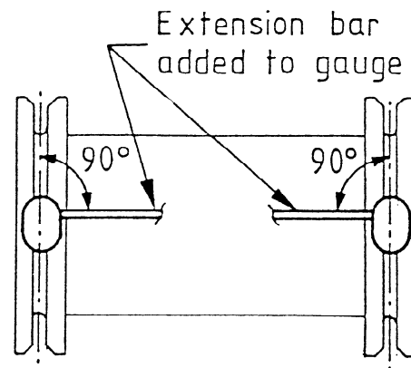
FIGURE 10 - Angular displacement of teeth across barrel
