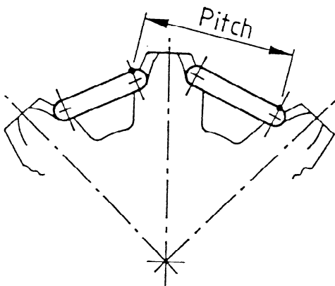
FIGURE 9 - Tooth pitch
