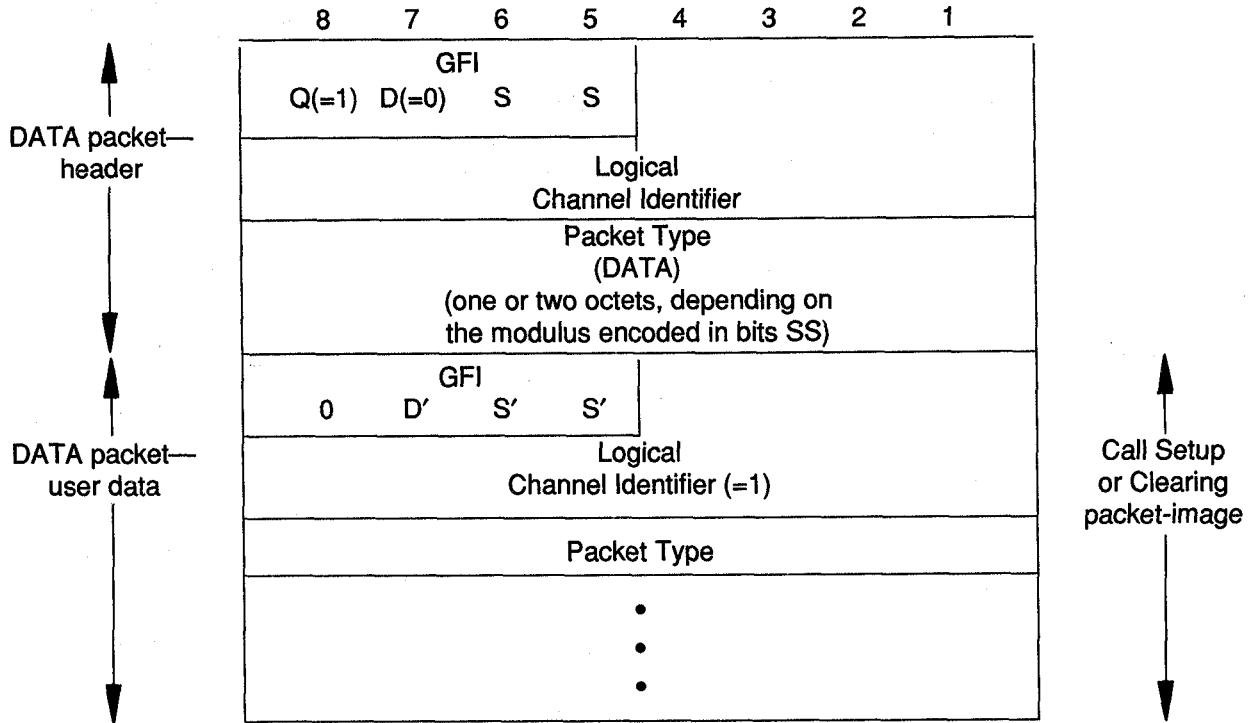
FIGURE 7 Call Setup/Clearing Encoding
