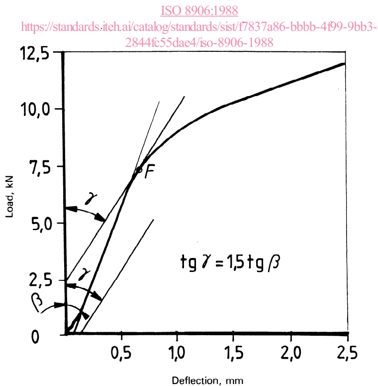
Figure 2 — "Load/deflection" curve
