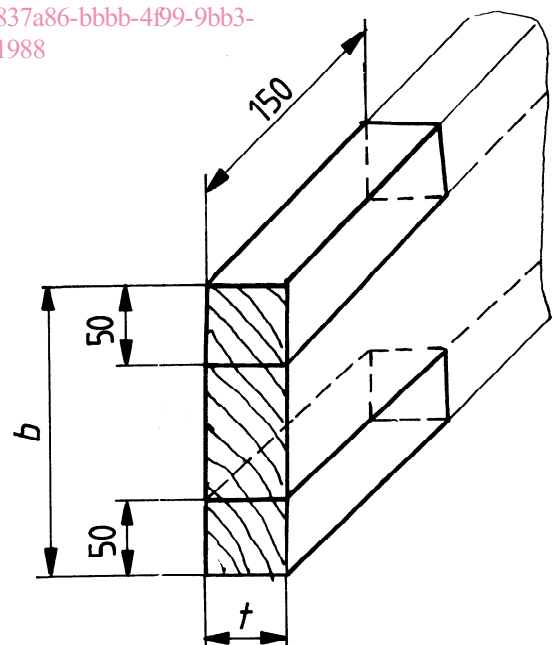
Figure 1 — Test pieces
