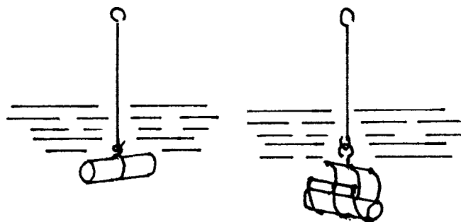
a. Twisted wire arrangement b. Basket support arrangement
