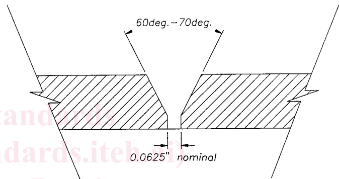
FIG. 1 Test Pieces
