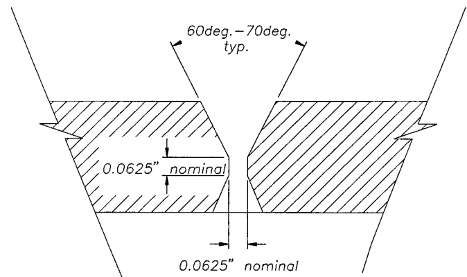
FIG. 2 Typical Bevel Profile (Sheet >0.090 to 0.5 in. (2.3 mm to 13 mm) in Thickness)
