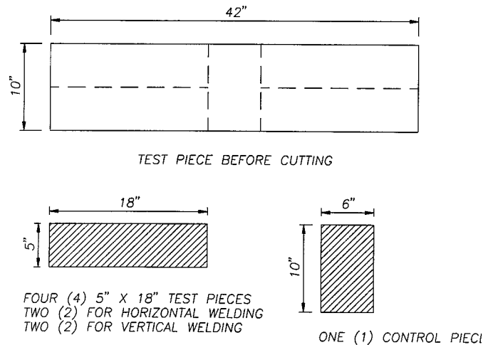
FIG. 1 Test Pieces
