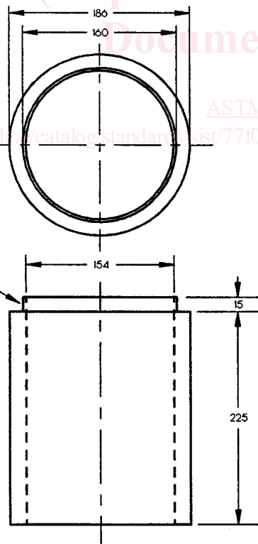
ALUMINUM CYLINDER TO SUPPORT PIPE ALL DIMENSIONS ARE mm UNLESS NOTED
