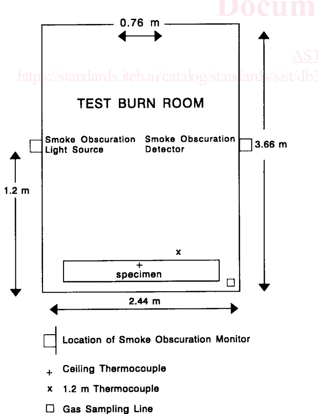
FIG. 1 Test Room Configuration A
