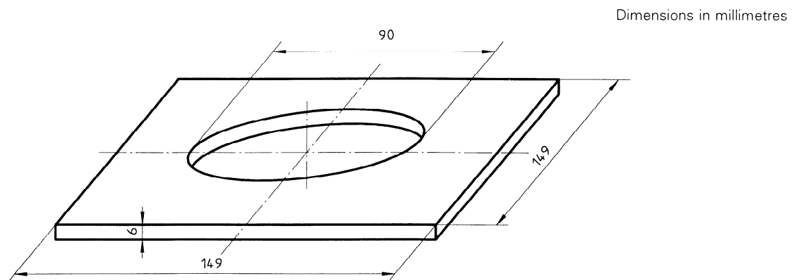
Figure 4 — Calorimeter location plate
