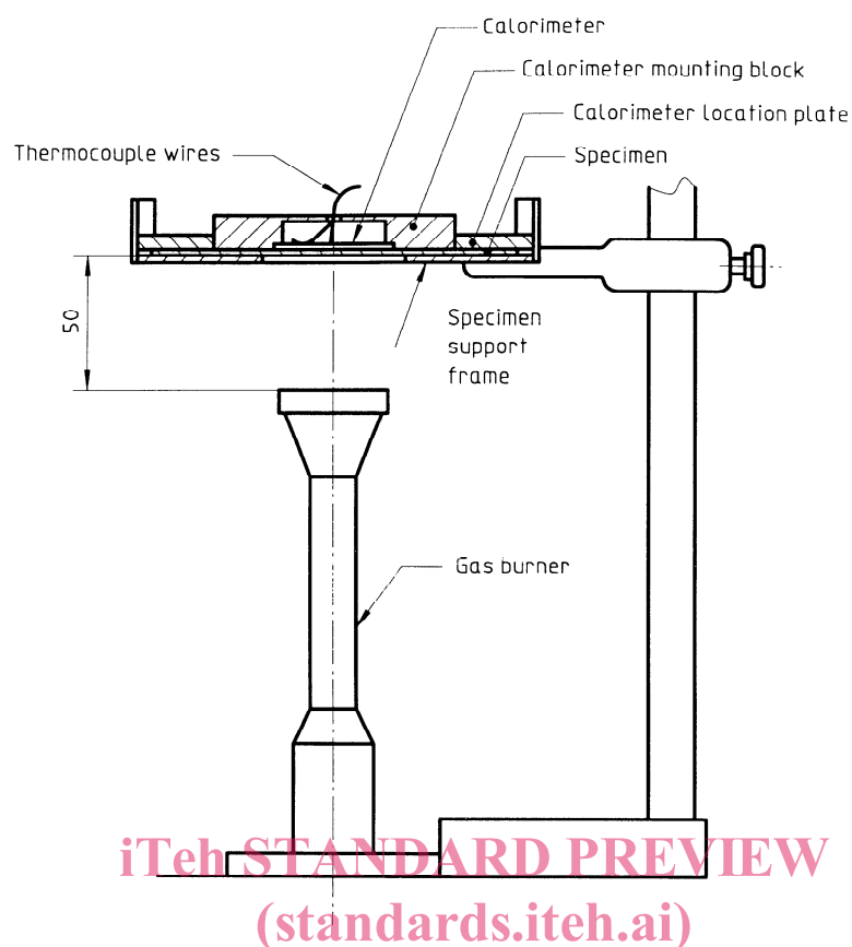
Figure 5 — Support stand
