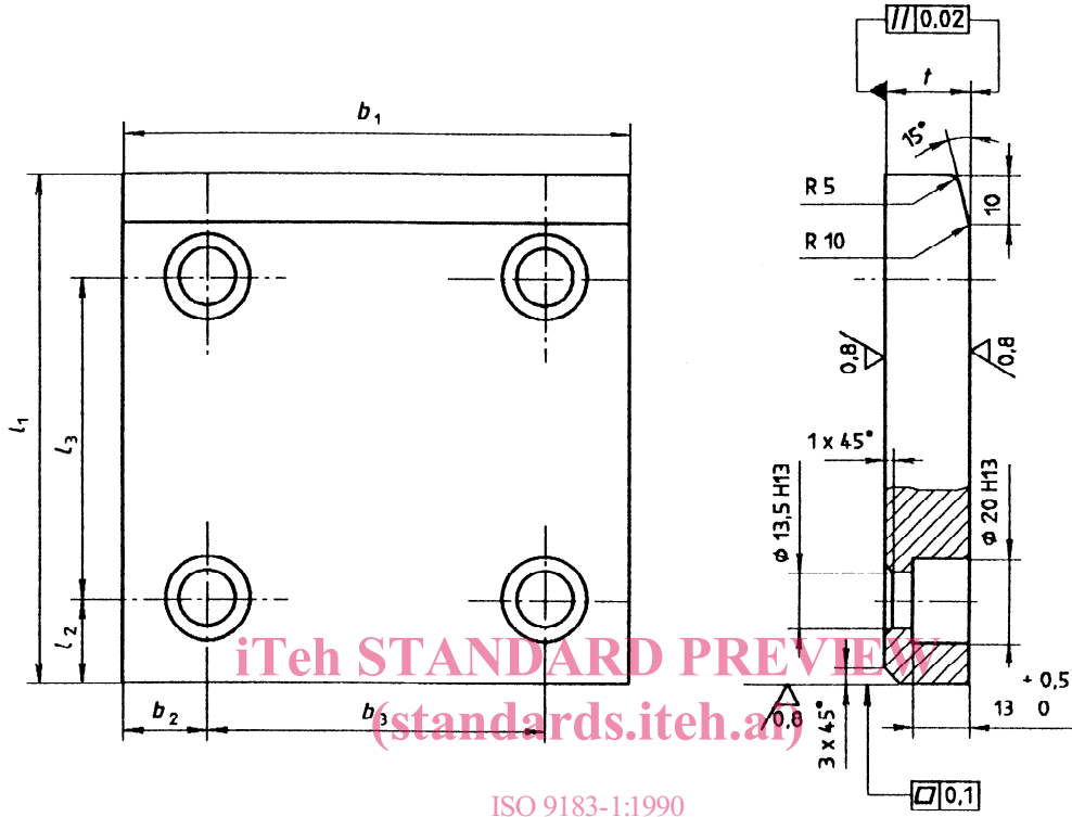
ISO 9183-1:1990 https://standards.iteh.ai/catalog/standards/sist/b9e08ebd-9c7b-43ce-8c95-82418cd391bc/iso-9183-1-1990 Figure 1 — Dimensions
