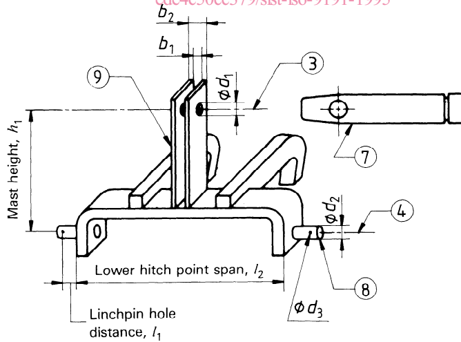
Figure 2 — Implement hitch
