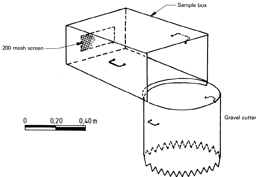
Figure 2 — Gravel-cutter sampler iTeh STANDARD PREVIEW (standards.iteh.ai)
