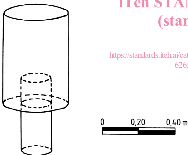
Figure 1 — Pipe sampler
